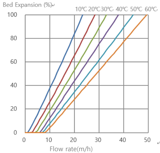
Figure 1. TRILITE® UPRC300U Bed Expansion
