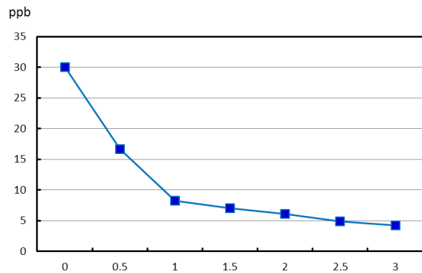
Figure 4. TRILITE® UPRC300U ΔTOC
