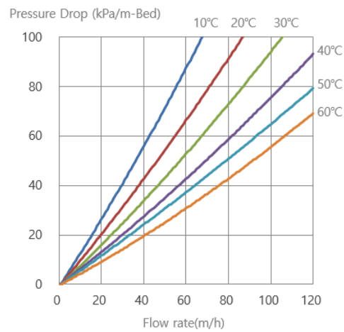
Figure 2. TRILITE® UPRC300U Drop Pressure
